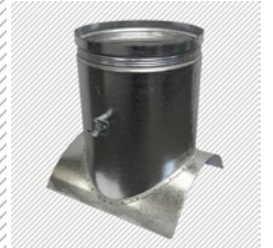
Saddle T/Off + Damper (Galvanised)
